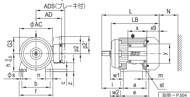
DRN200 - 225, DRN315
