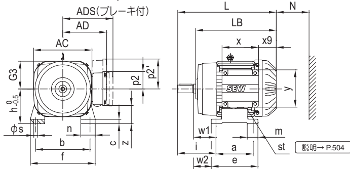
DRN132M - 180, DRN250 - 280
