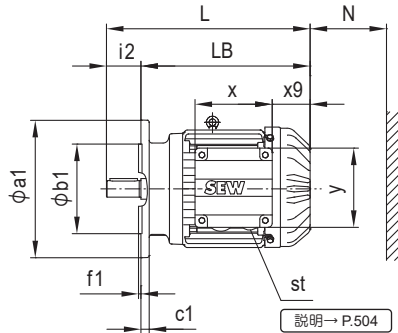
DR2S63 - 200
