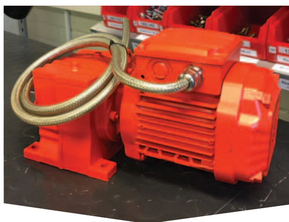
SmartStart motor cable incl. EMC cable gland, motor cable and installation star/delta.
